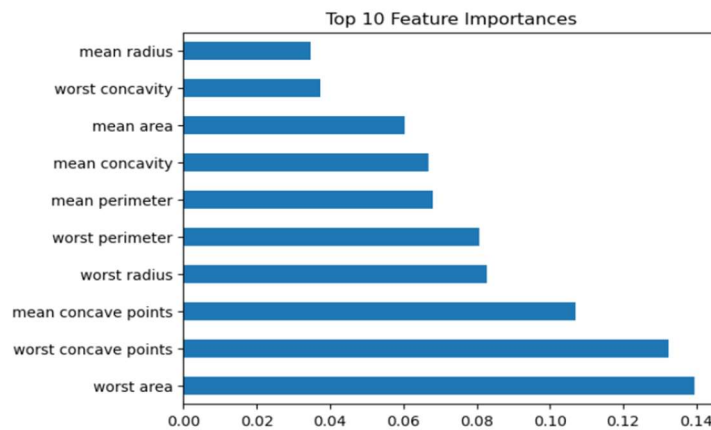
Fig 6.6 – Feature Selection
